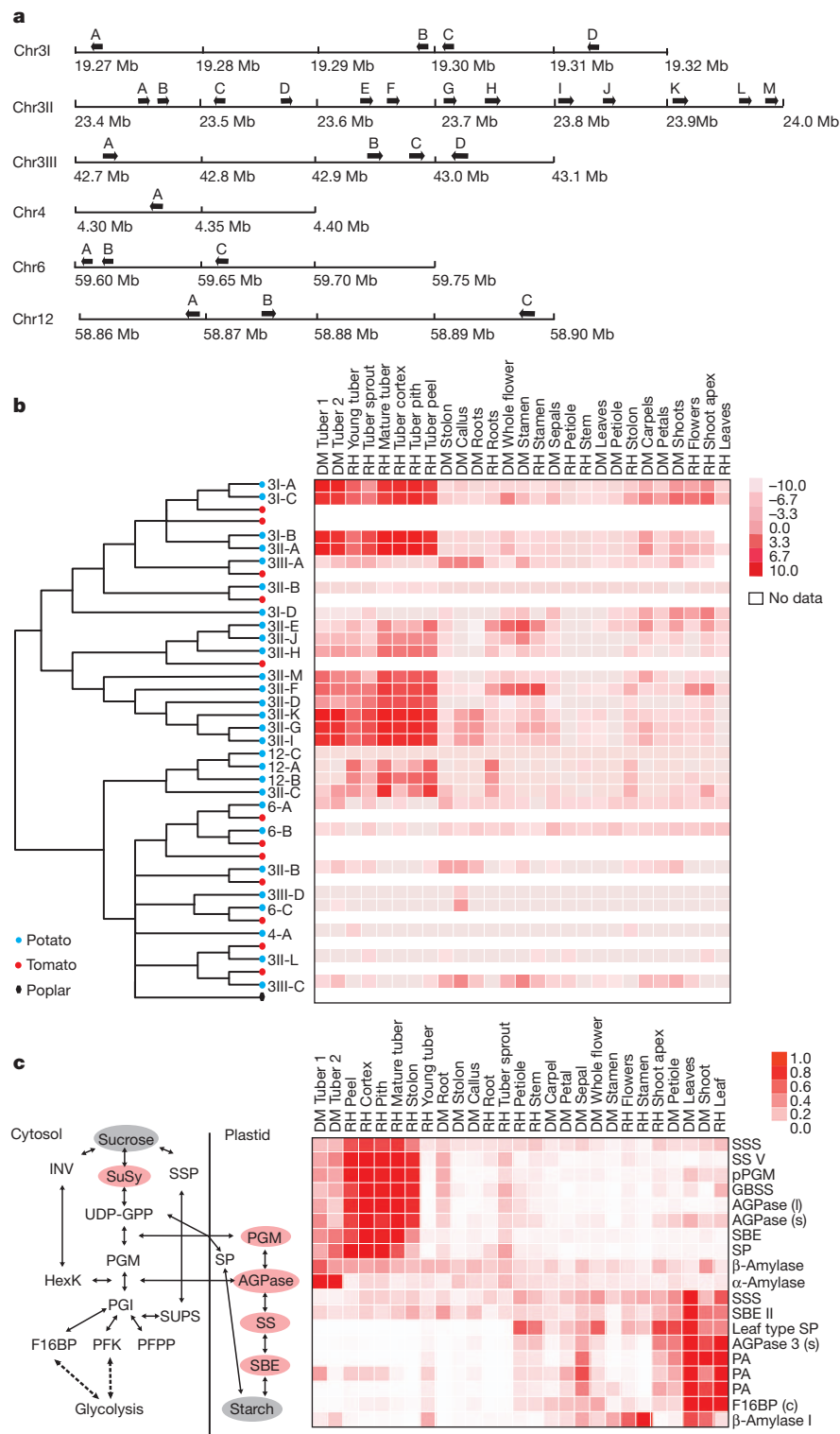
Figure 4 | Gene expression of selected tissues and genes. a , KTI gene organization across the potato genome. Black arrows indicate the location of individual genes on six scaffolds located on four chromosomes. b , Phylogenetic tree and KTI gene expression heat map. The KTI genes were clustered using all potato and tomato genes available with the Populus KTI gene as an out-group. The tissue specificity of individual members of the highly expanded potato gene family is shown in the heat map. Expression levels are indicated by shades of red, where white indicates no expression or lack of data for tomato and poplar. c , A model of starch synthesis showing enzyme activities is shown on the left. AGPase, ADP-glucose pyrophosphorylase; F16BP, fructose-1,6-biphosphatase; HexK, hexokinase; INV, invertase; PFK, phosphofructokinase; PFPP, pyrophosphate-fructose-6-phosphate-1-phosphotransferase; PGI, phosphoglucose isomerase; PGM, phosphoglucomutase; SBE, starch branching enzyme; SP, starch phosphorylase; SPP, sucrose phosphate phosphatase; SS, starch synthase; SuSy, sucrose synthase; SUPS, sucrose phosphate synthase; UDP-GPP, UDP-glucose pyrophosphorylase. The grey background denotes substrate (sucrose) and product (starch) and the red background indicates genes that are specifically upregulated in RH versus DM. On the right, a heat map of the genes involved in carbohydrate metabolism is shown. ADP-glucose pyrophosphorylase large subunit, AGPase (I); ADP-glucose pyrophosphorylase small subunit, AGPase (s); ADP-glucose pyrophosphorylase small subunit 3, AGPase 3 (s); cytosolic fructose-1,6-biphosphatase, F16BP (c); granule bound starch synthase, GBSS; leaf type L starch phosphorylase, Leaf type SP; plastidic phosphoglucomutase, pPGM; starch branching enzyme II, SBE II; soluble starch synthase, SSS; starch synthase V, SSV; three variants of plastidic aldolase, PA.
